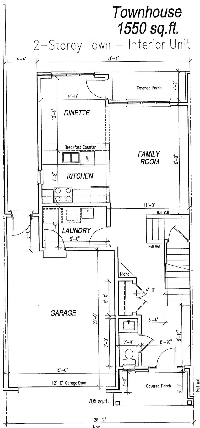
Main Floor Plan 9'-0" Main Floor Ceiling Height
