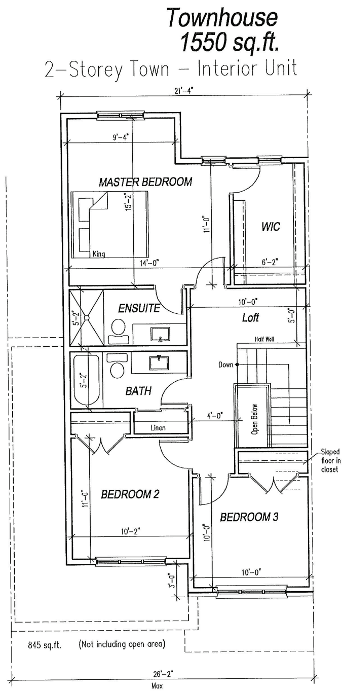
Second Floor Plan 8'-0" Second Floor Ceiling Height
