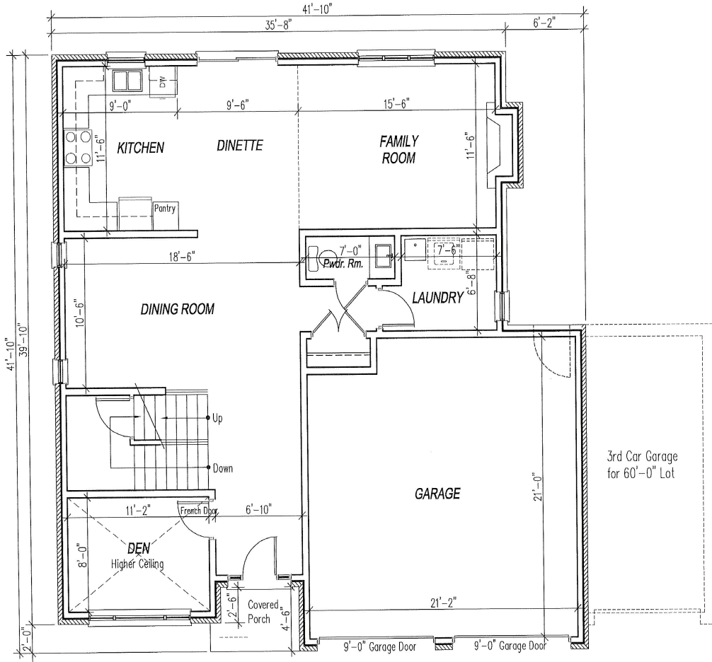
Main Floor Plan 1100 sq.ft. 9'-0" Main Floor Ceiling Height
