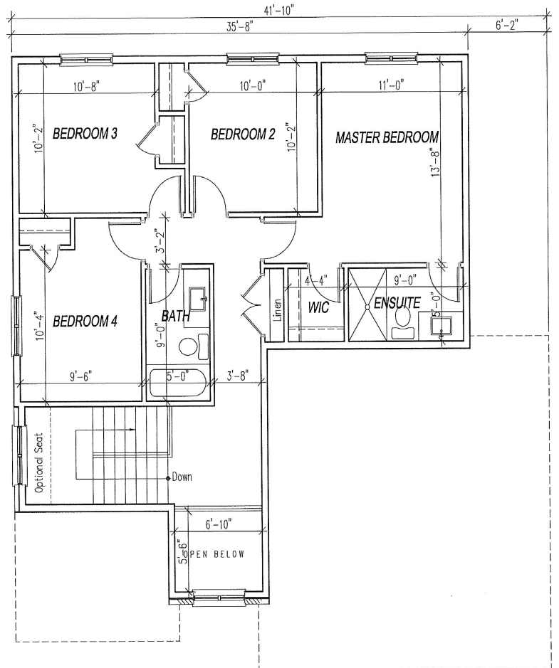
Second Floor Plan 930 sq.ft. (not including open area) 8'-0" Second Floor Ceiling Height
