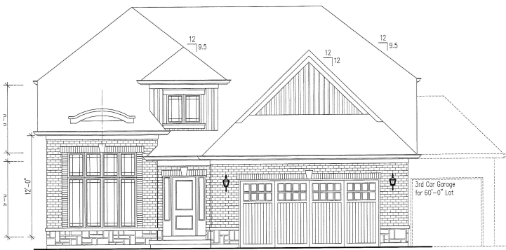
Front Elevation Elevation 'A'
